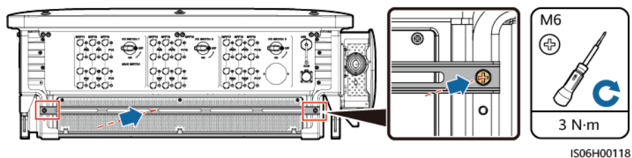
Figura A-5 Installing a beam
