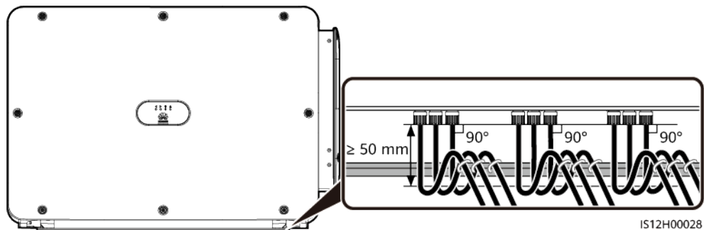
Figura A-6 Binding Y-branch connectors
