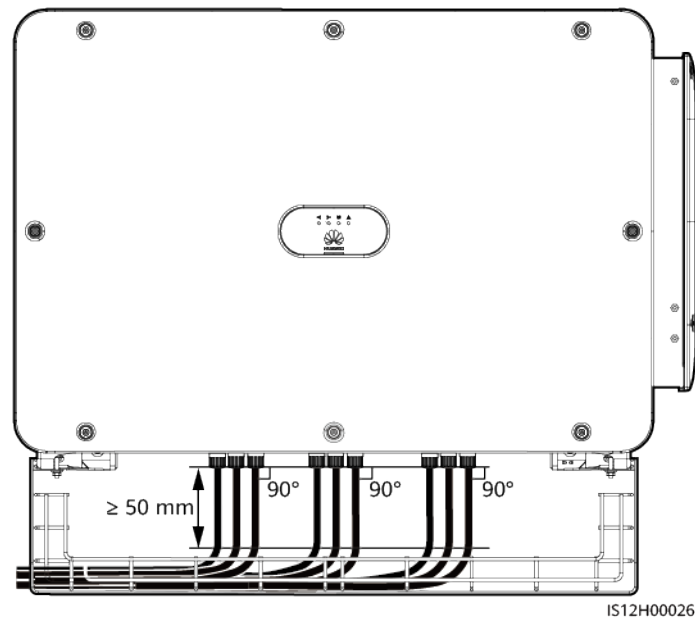
Figura A-3 Placing Y-branch connectors
