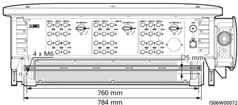
Figura A-4 Recommended dimensions
